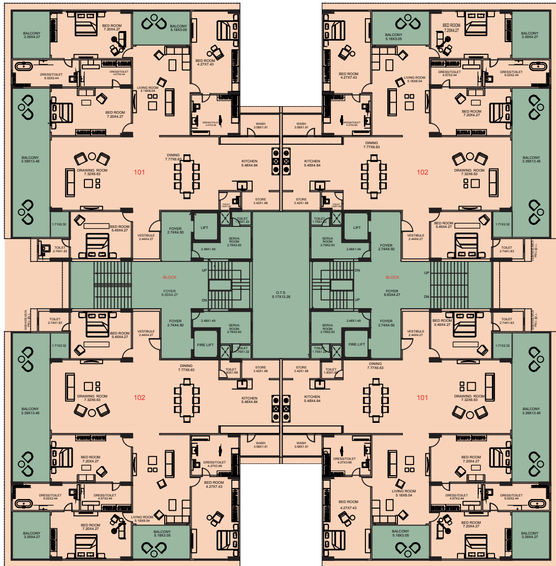
2ND to 13TH FLOOR PLAN
