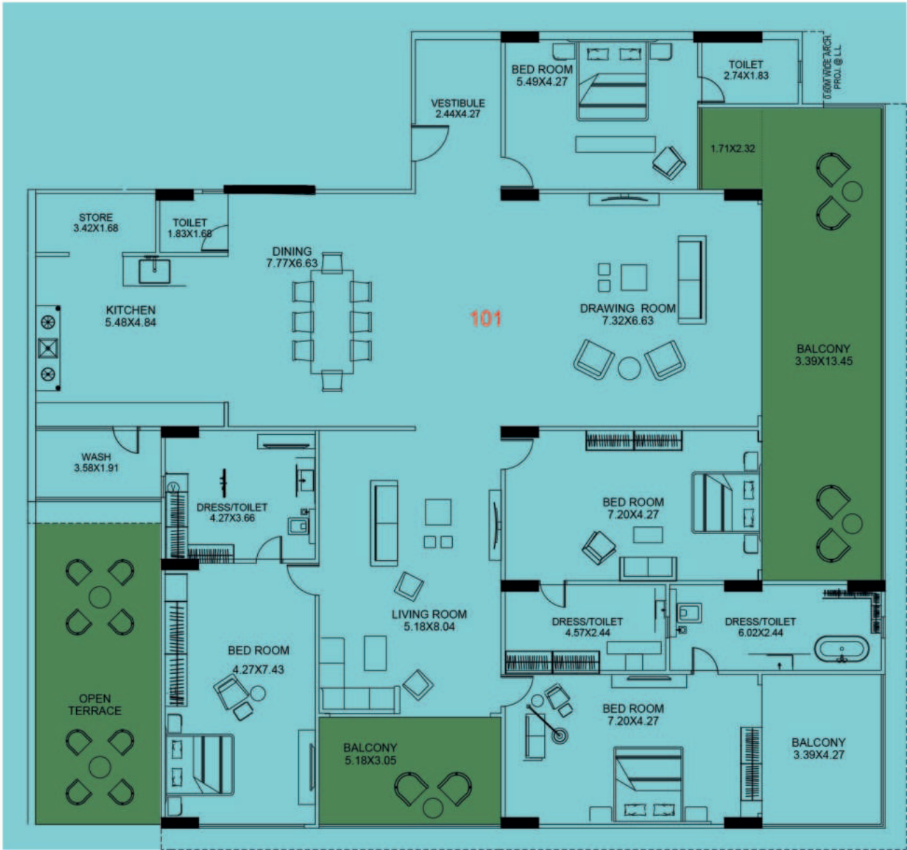
UNIT PLAN
