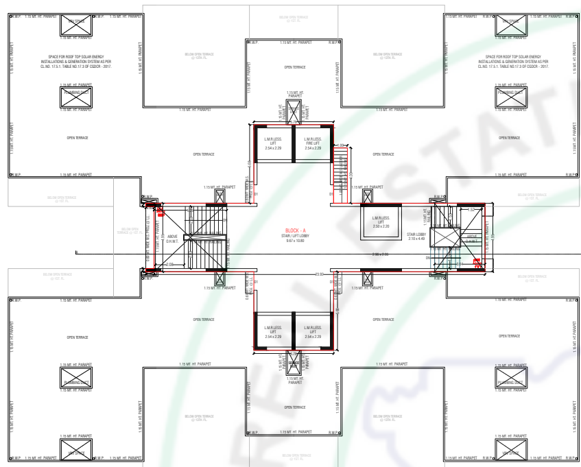
OPEN TERRACE PLAN WITH STAIR CABBIN & O.H.W.T.
