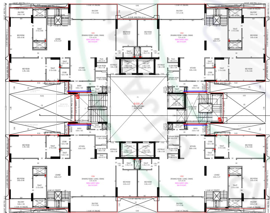
12TH FLOOR PLAN
