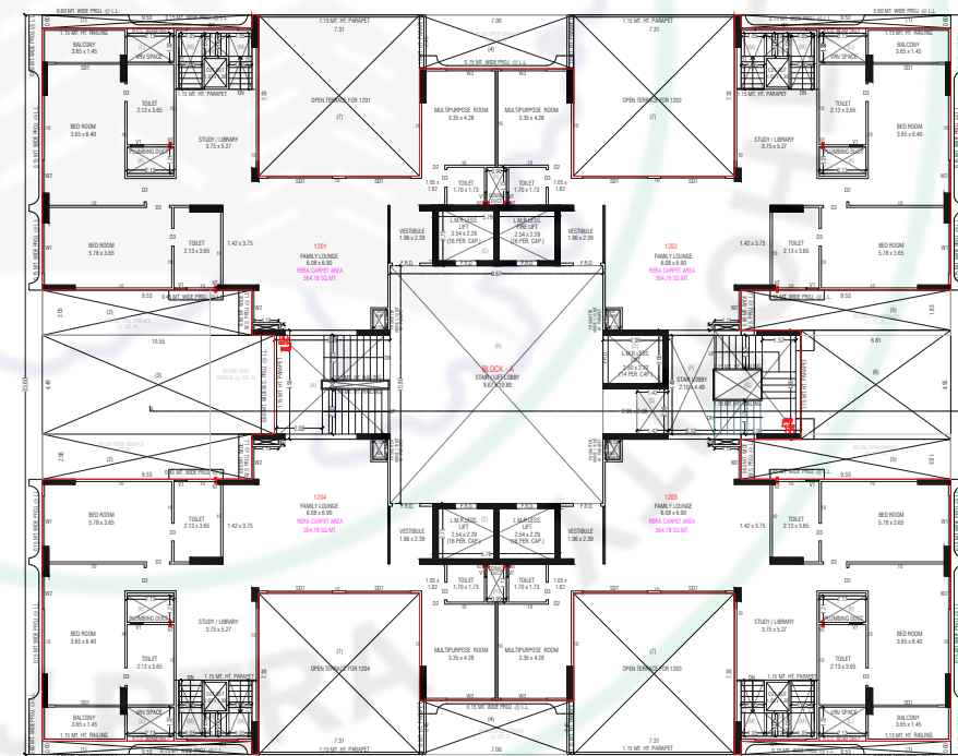
13TH FLOOR PLAN
