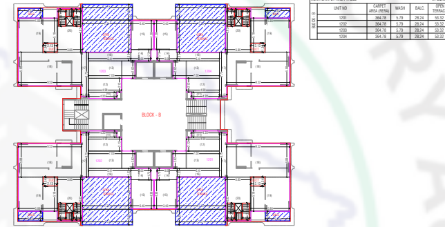
NET CARPET AREA CALC. - 18TH FLOOR PLAN (SCALE - 1:500) - 2000 MET
