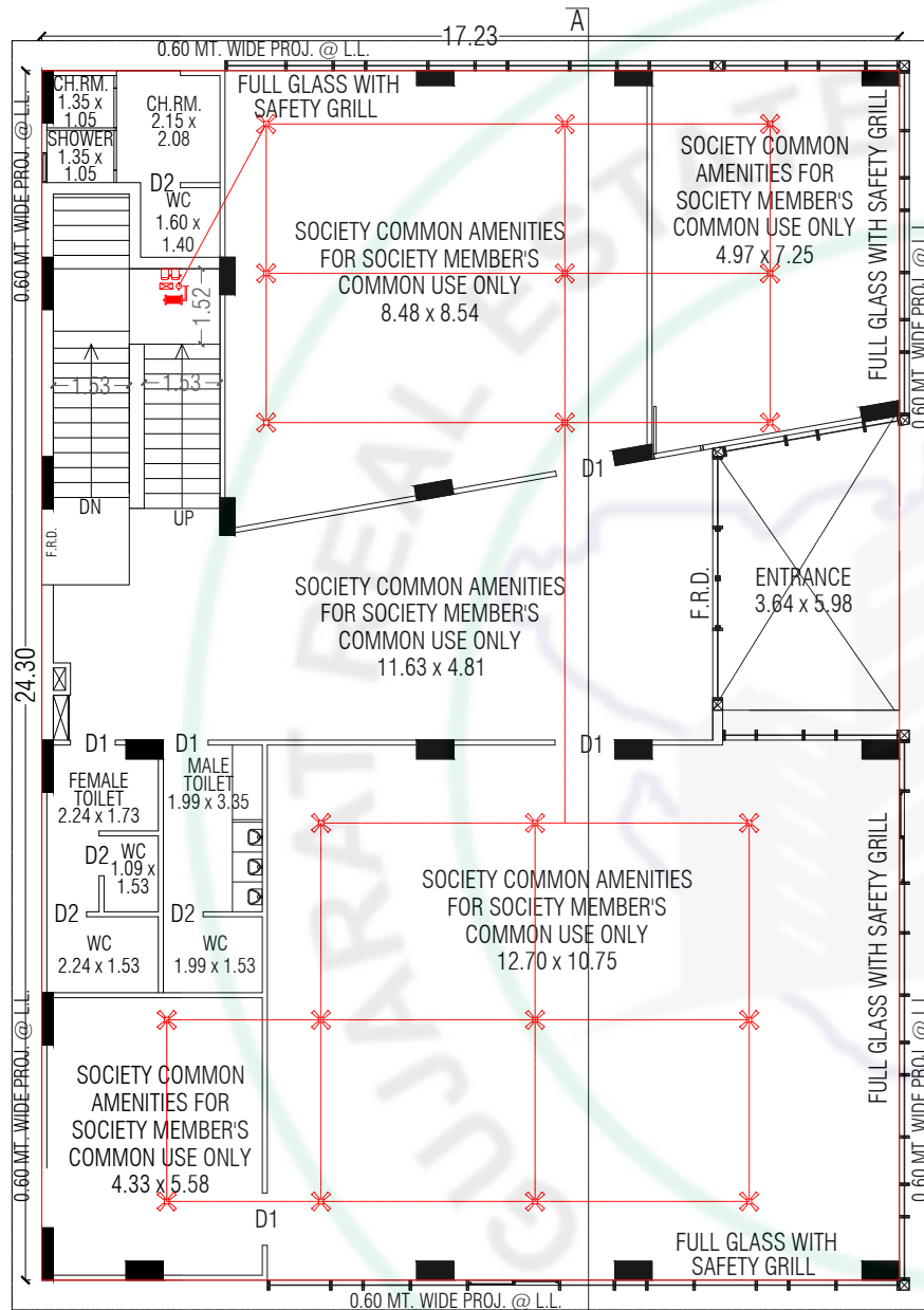
GR. FL. PLAN SOCIETY COMMON AMENITIES FOR SOCIETY
