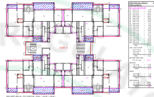
NET CARPET AREA CALC. - 17TH FLOOR PLAN (SCALE - 1:500) - 2000 MET
